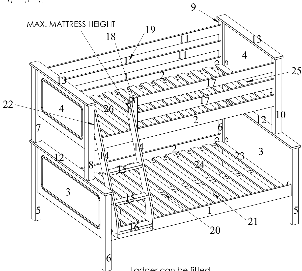
LADDER LEFT
